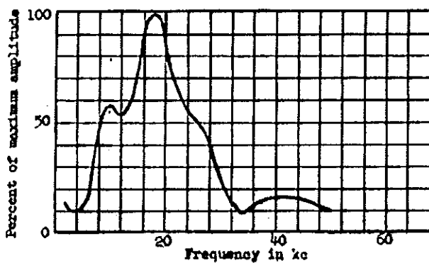
Fig. 3.82 Frequency function of broadband pulse Shot No. 8 1000 km from ground zero
